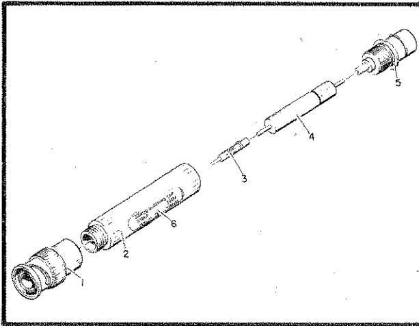
Figure 2. Model 10240B Parts
